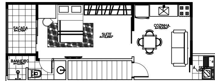
LAYOUT escala.....1:50
